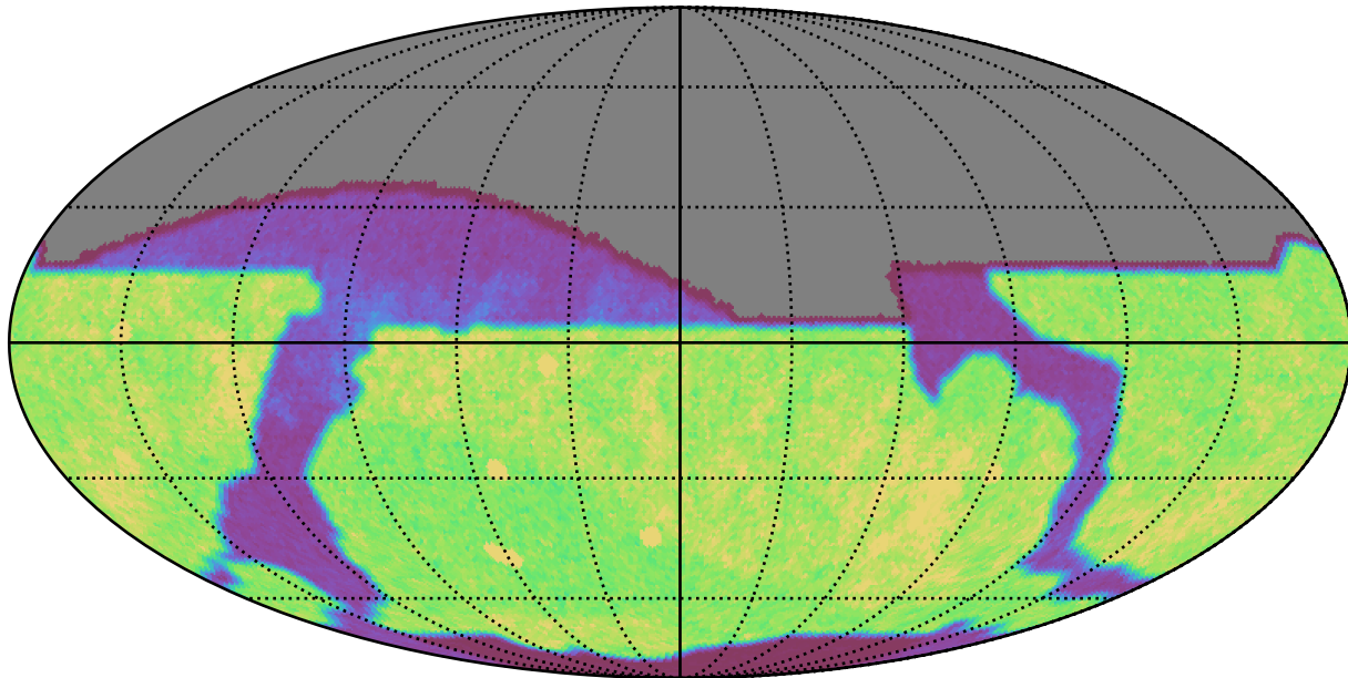
weather_cloudso31v3.5_10yrs i: Count observationStartMJD
