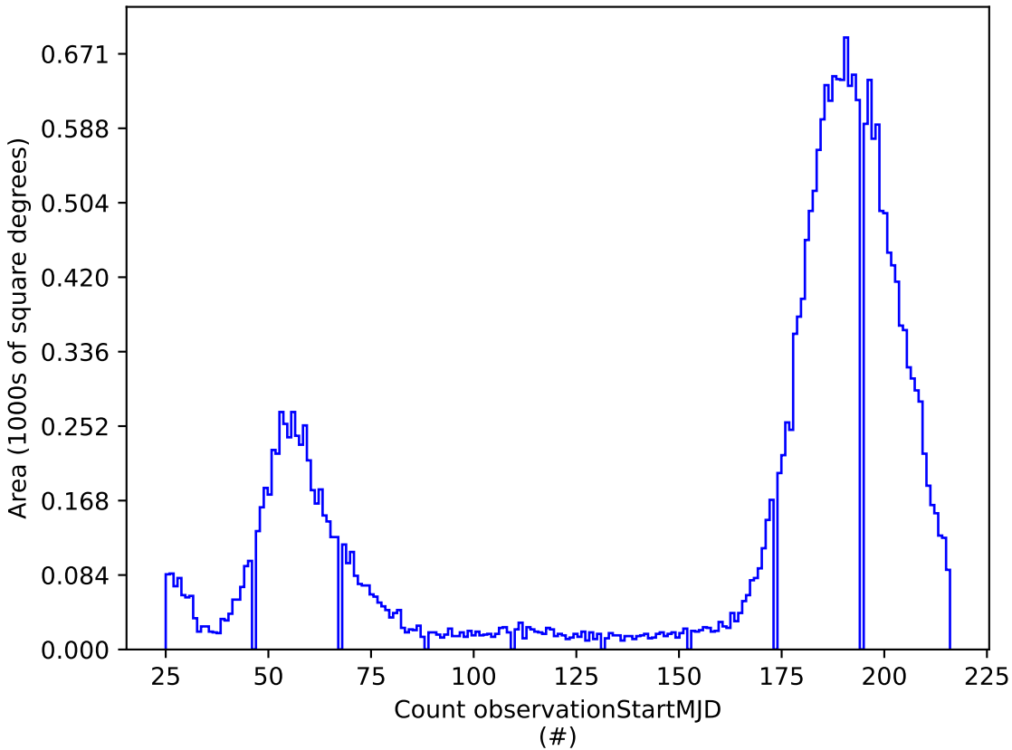
weather_cloudso31v3.5_10yrs r: Count observationStartMJD
