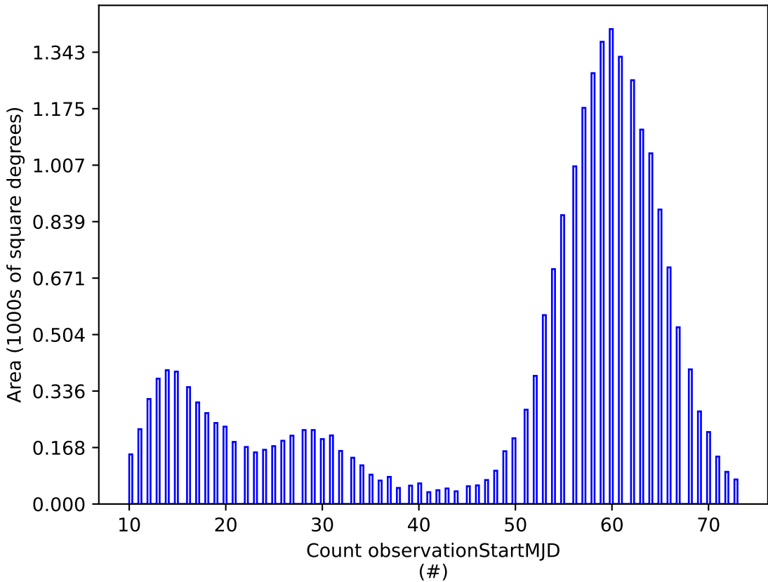
weather_cloudso31v3.5_10yrs u: Count observationStartMJD
