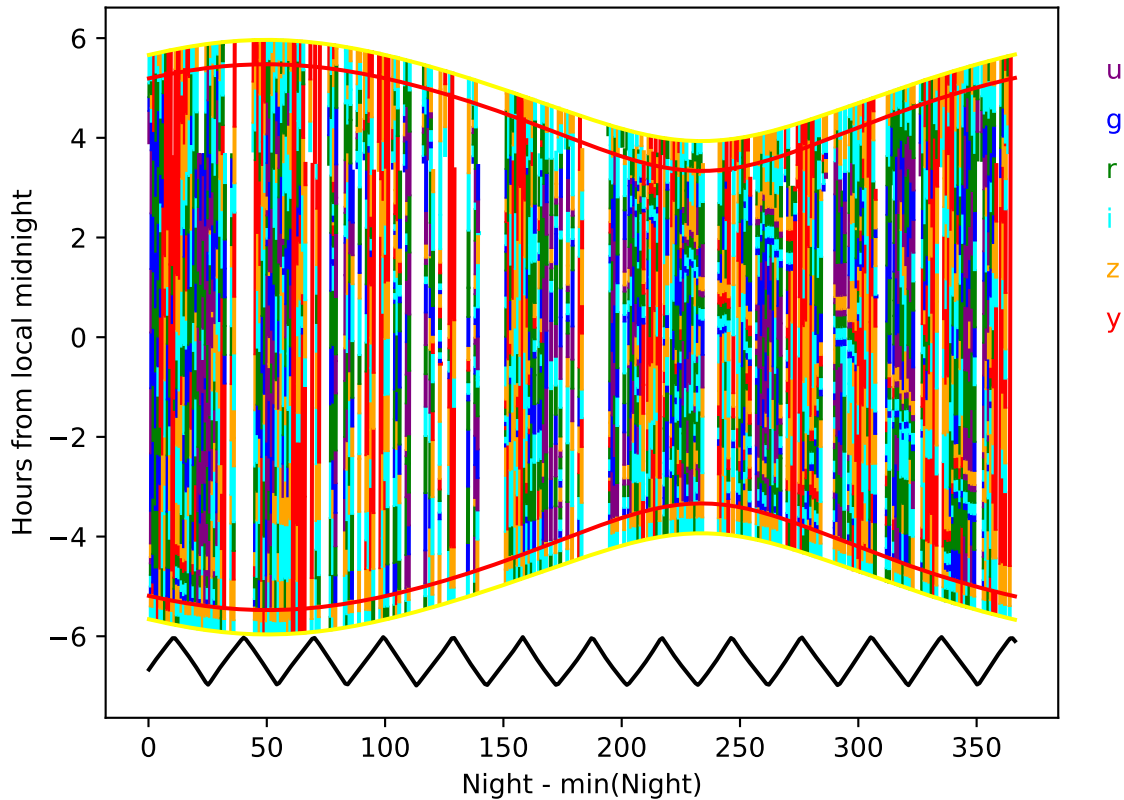
weather_cloudso31v3.5_10yrs year 0-1: Hourglass
