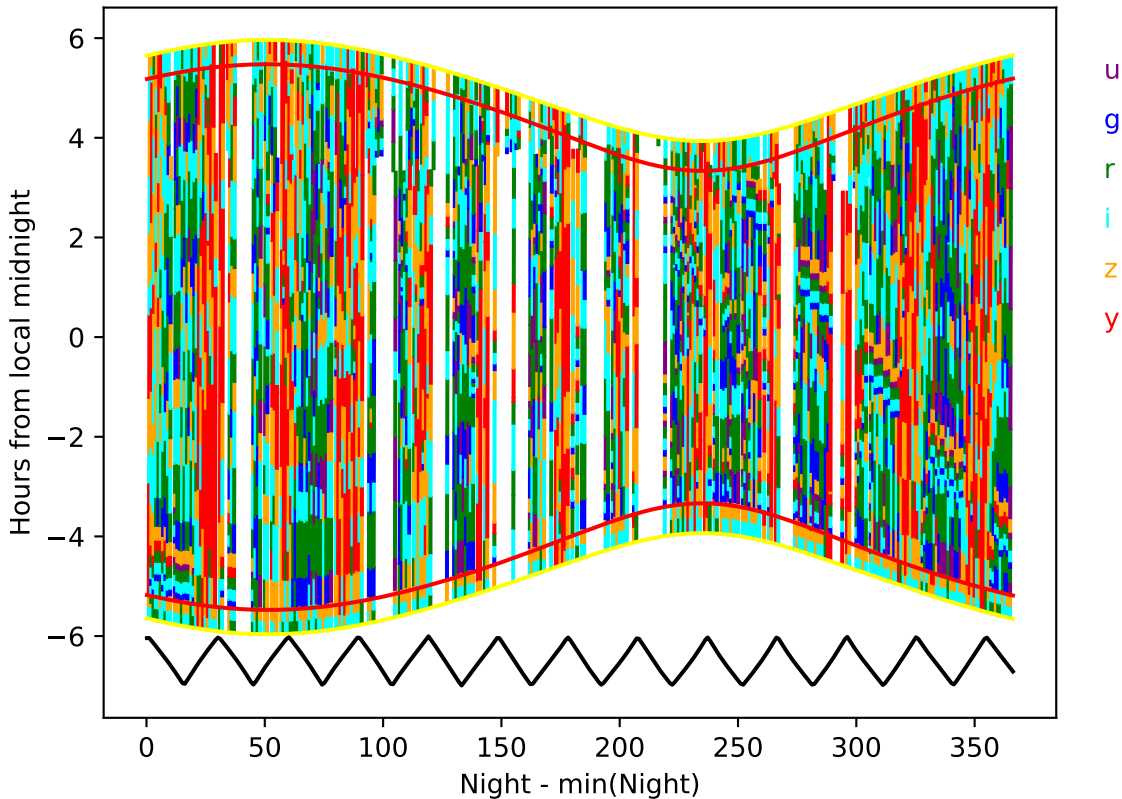
weather_cloudso31v3.5_10yrs year 1-2: Hourglass
