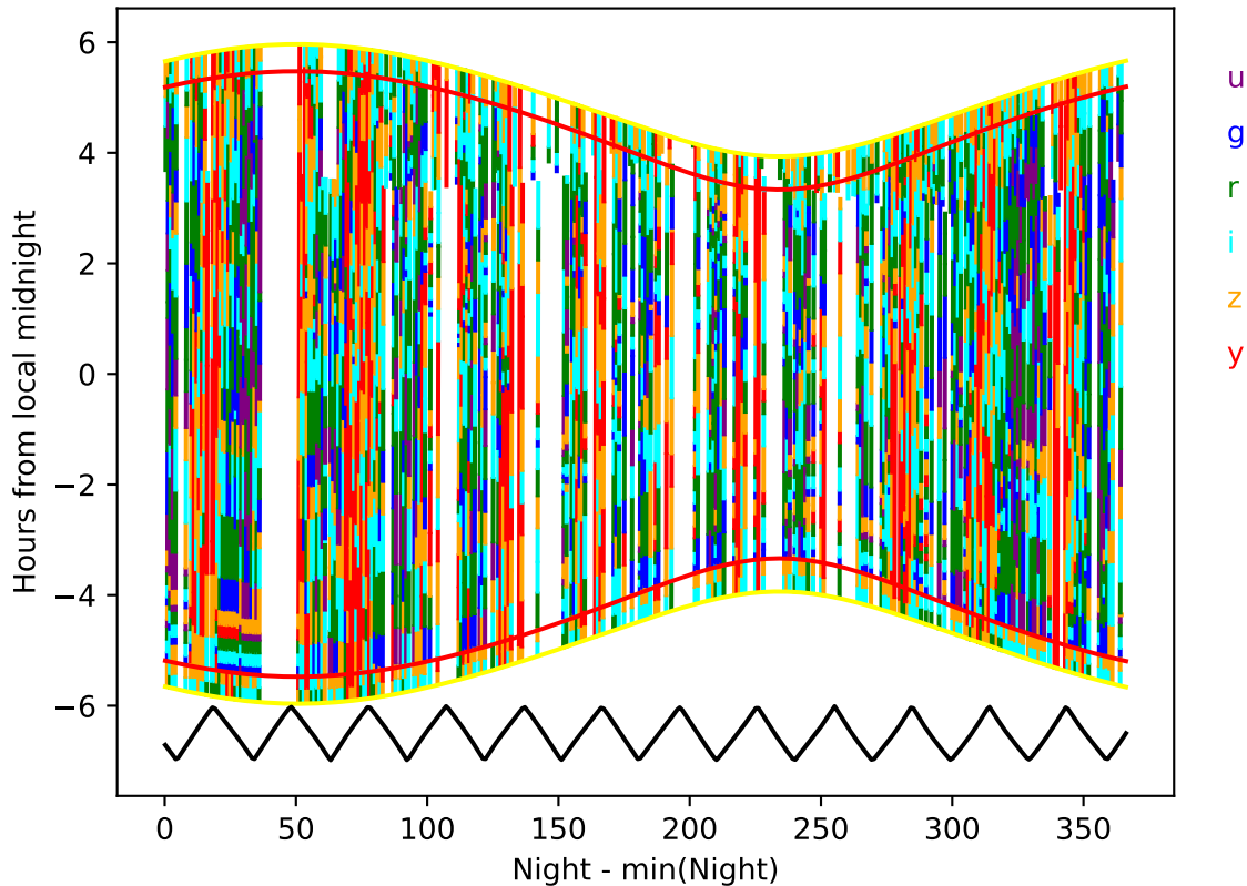
weather_cloudso31v3.5_10yrs year 2-3: Hourglass
