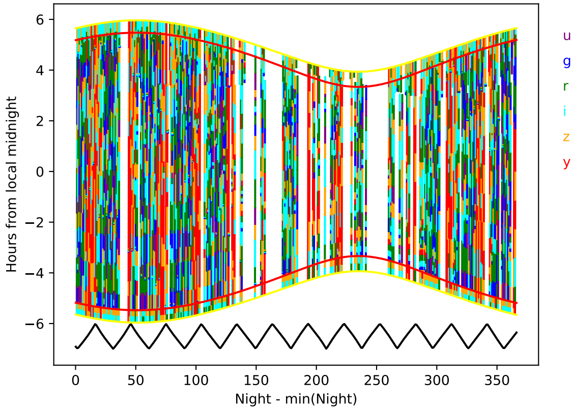
weather_cloudso31v3.5_10yrs year 5-6: Hourglass
