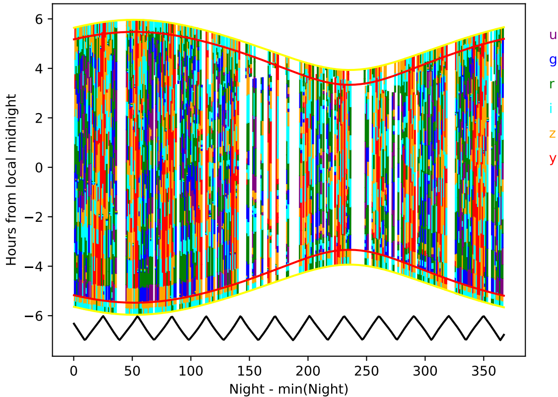
weather_cloudso31v3.5_10yrs year 7-8: Hourglass
