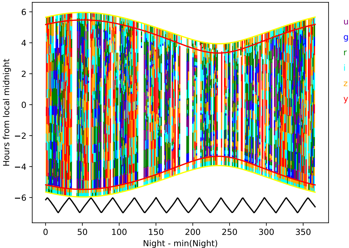
weather_cloudso31v3.5_10yrs year 9-10: Hourglass
