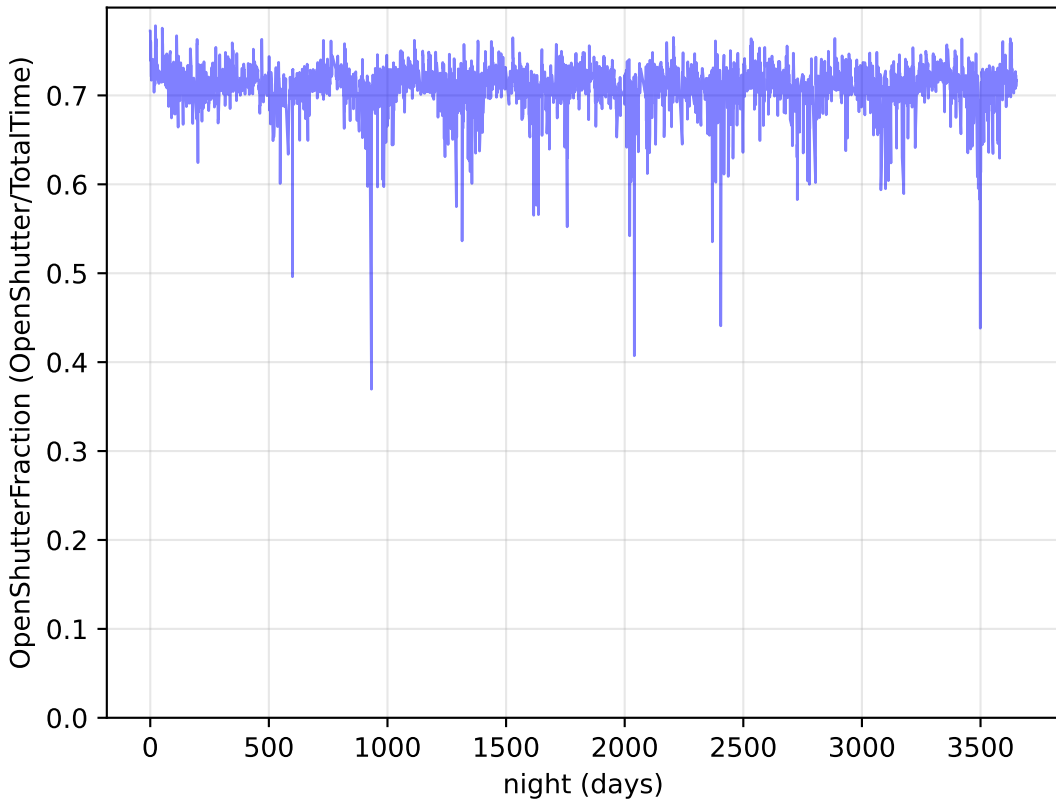
weather_cloudso31v3.5_10yrs : OpenShutterFraction
