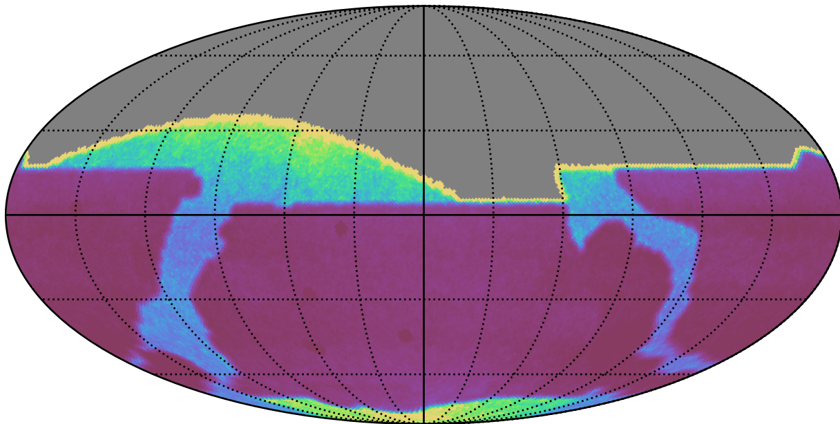
weather_cloudso31v3.5_10yrs : properMotion
