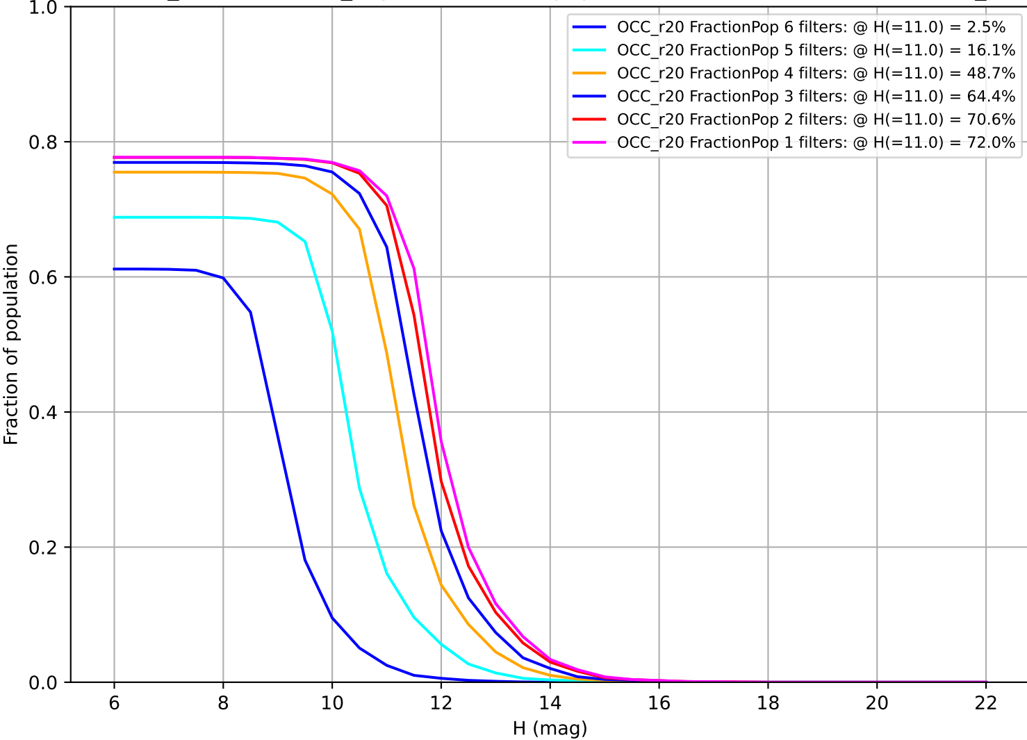
weather_cloudso31v3.5_10yrs: Fraction of population with colors in X filters OCC_r20
