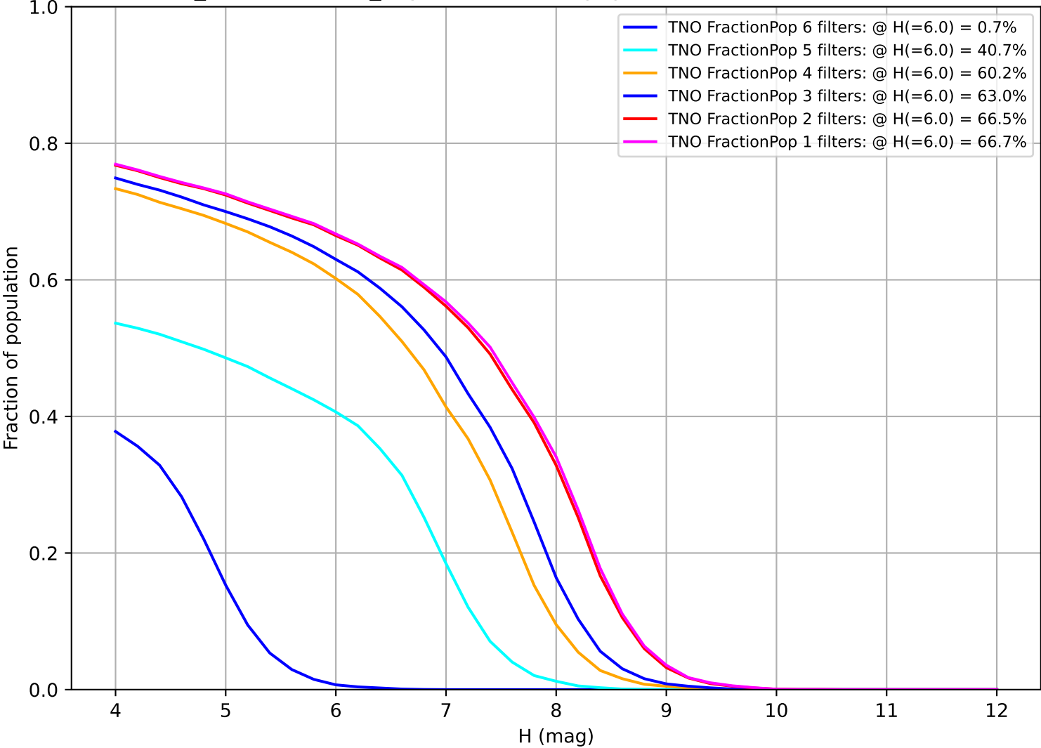
weather_cloudso31v3.5_10yrs: Fraction of population with colors in X filters TNO
