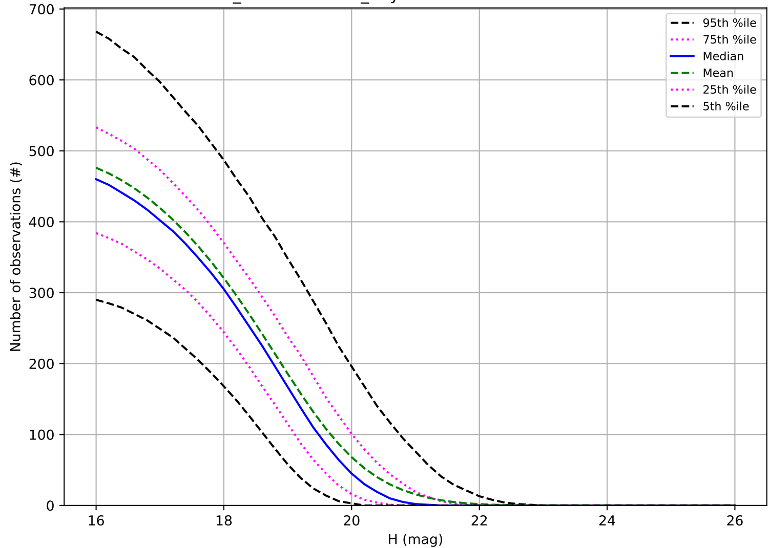
weather_cloudso31v3.5_10yrs: Number of observations MBA
