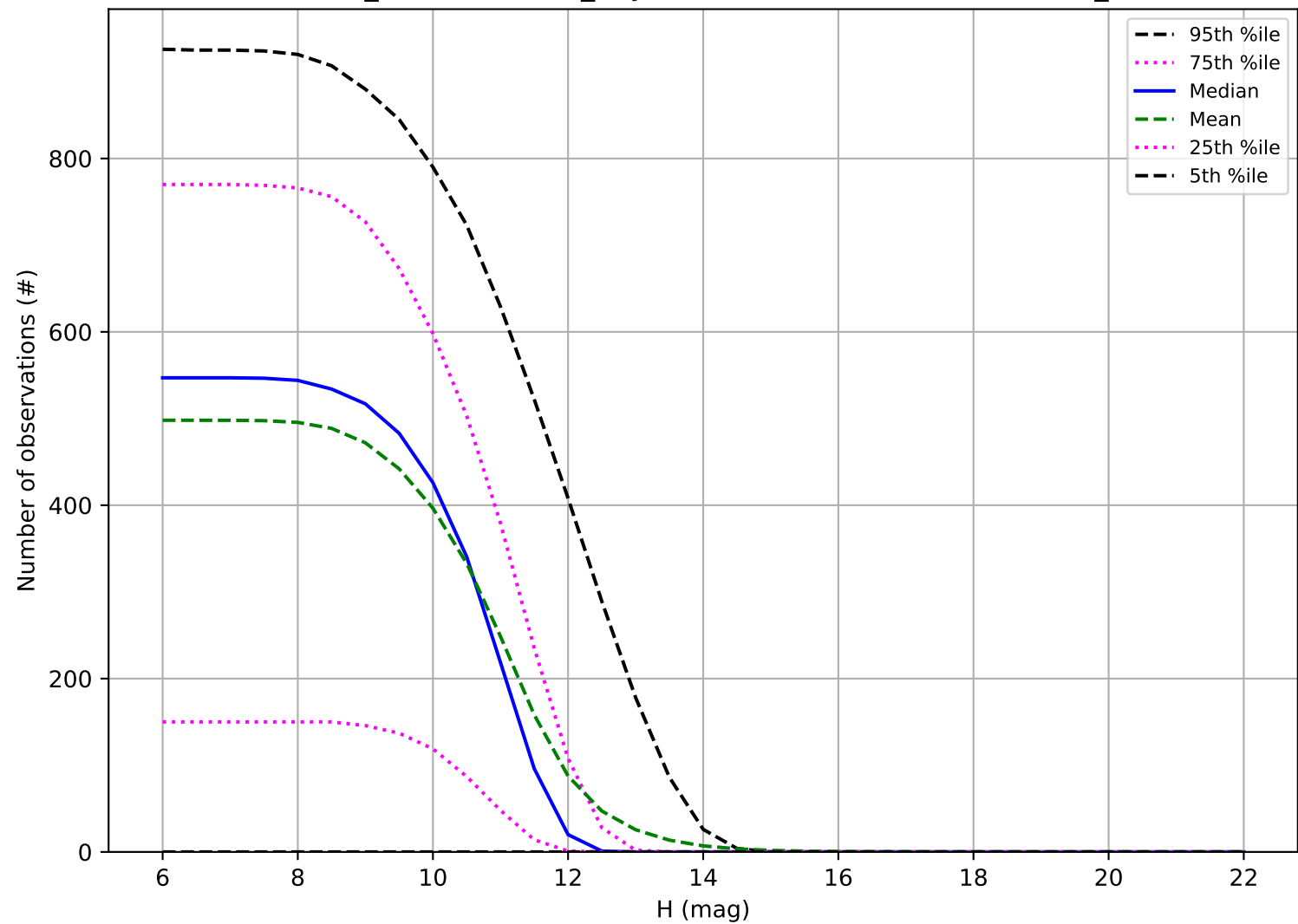
weather_cloudso31v3.5_10yrs: Number of observations OCC_r20
