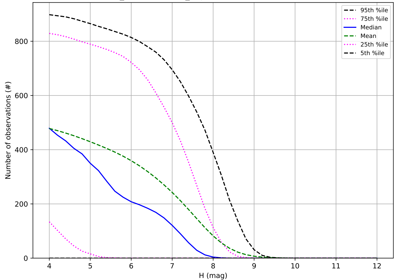
weather_cloudso31v3.5_10yrs: Number of observations TNO
