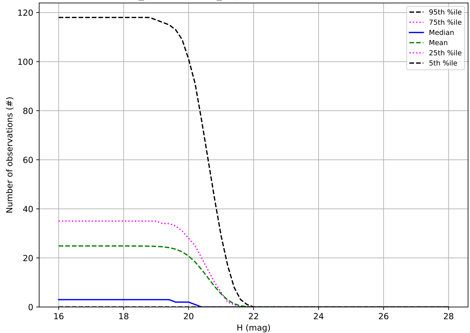
weather_cloudso31v3.5_10yrs: Number of observations Vatira
