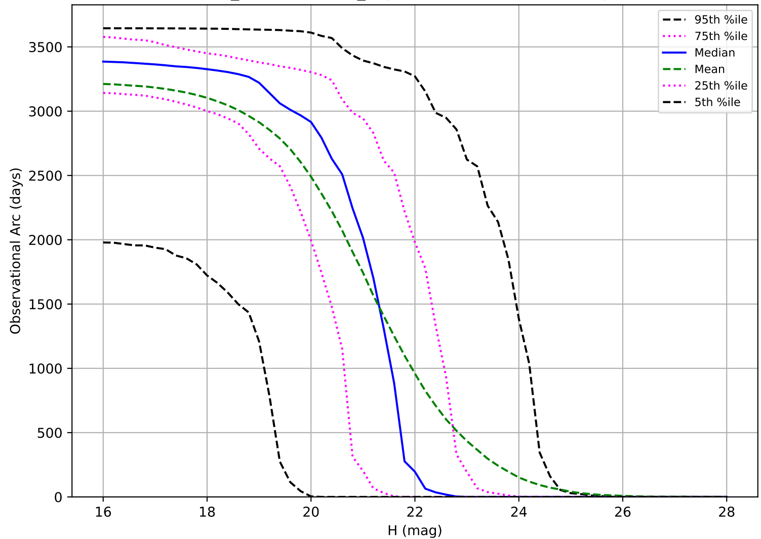
weather_cloudso31v3.5_10yrs: Observational Arc Length PHA
