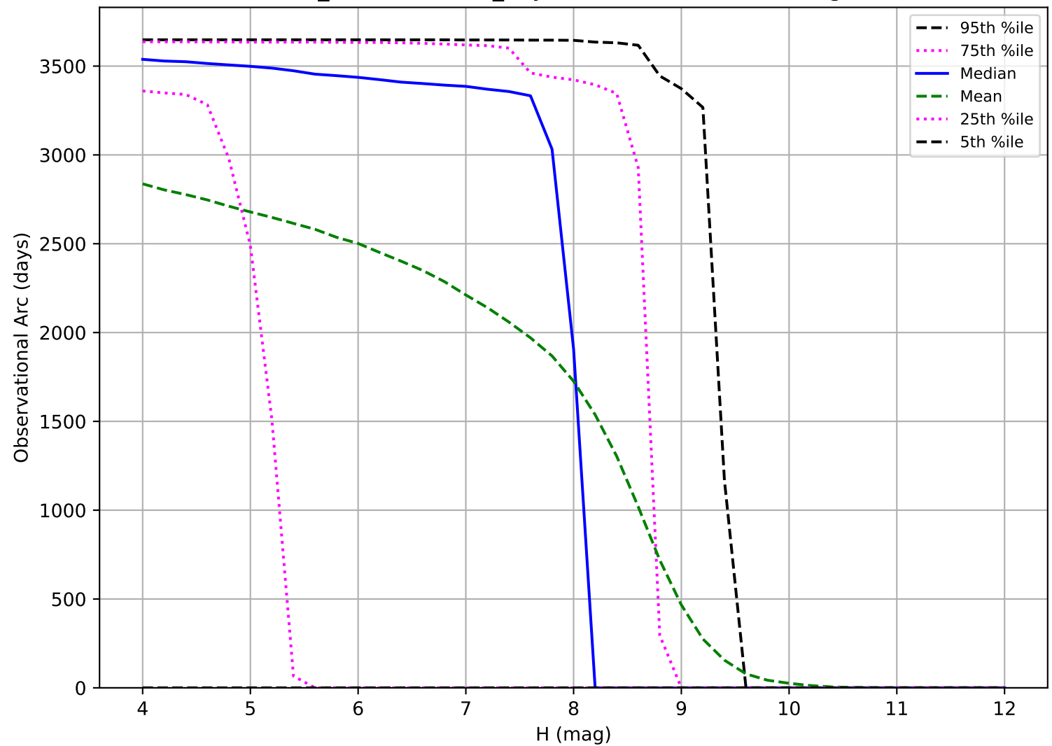
weather_cloudso31v3.5_10yrs: Observational Arc Length TNO
