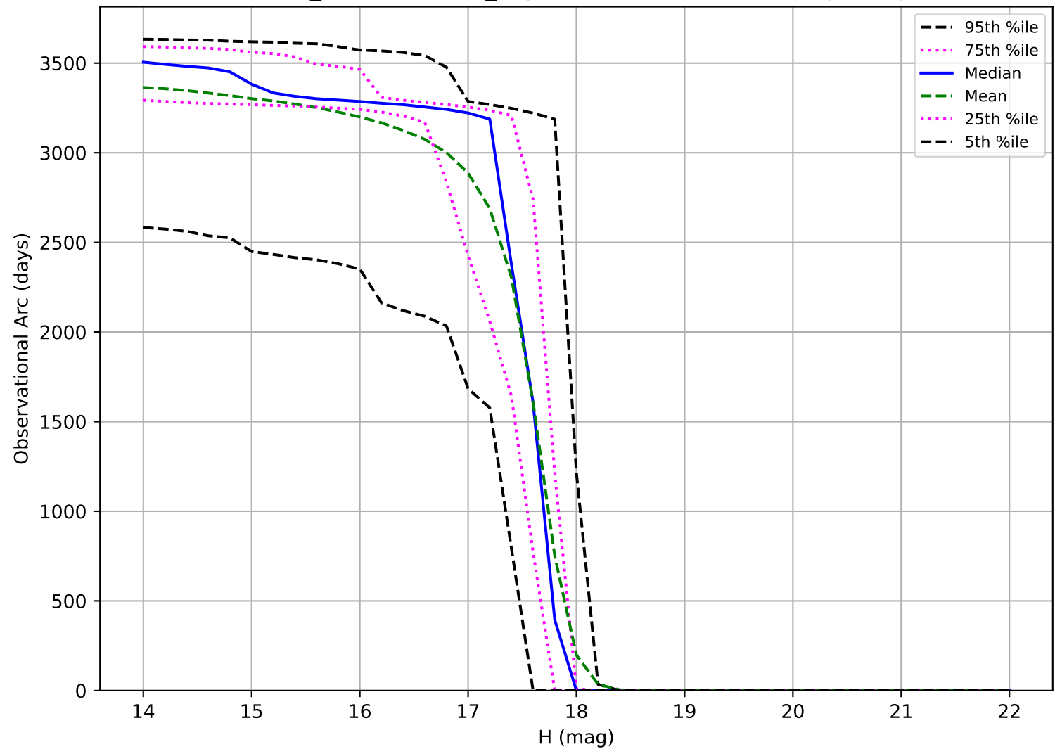
weather_cloudso31v3.5_10yrs: Observational Arc Length Trojan
