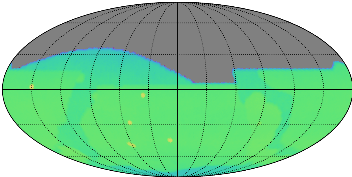
weather_cloudso35v3.5_10yrs : CoaddM5
