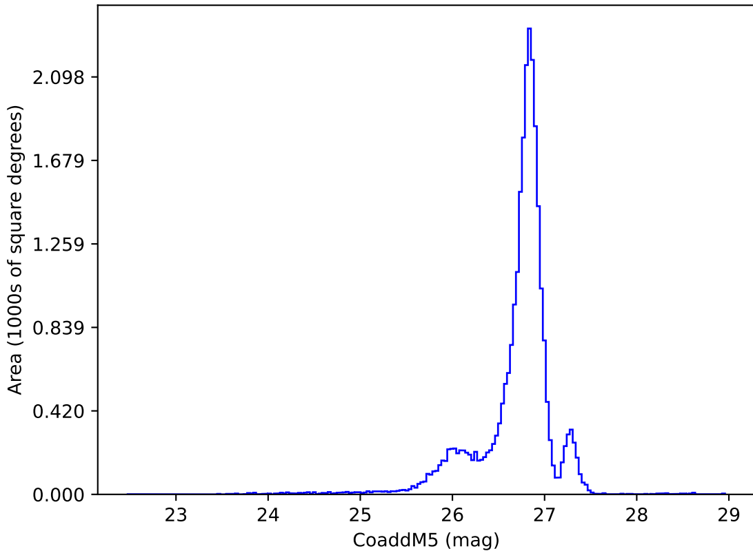
weather_cloudso35v3.5_10yrs g: CoaddM5
