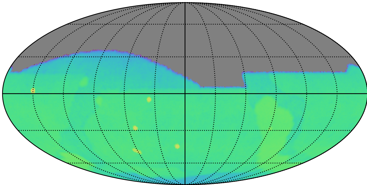
weather_cloudso35v3.5_10yrs g: CoaddM5
