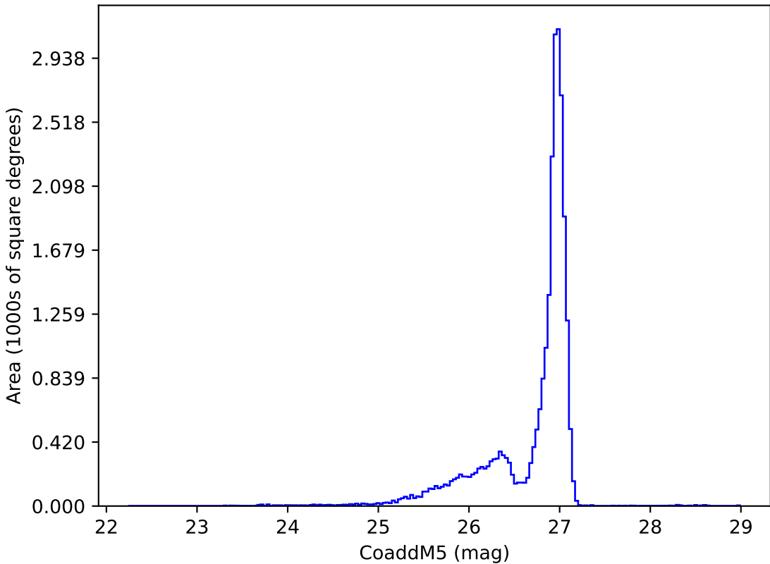
weather_cloudso35v3.5_10yrs r: CoaddM5
