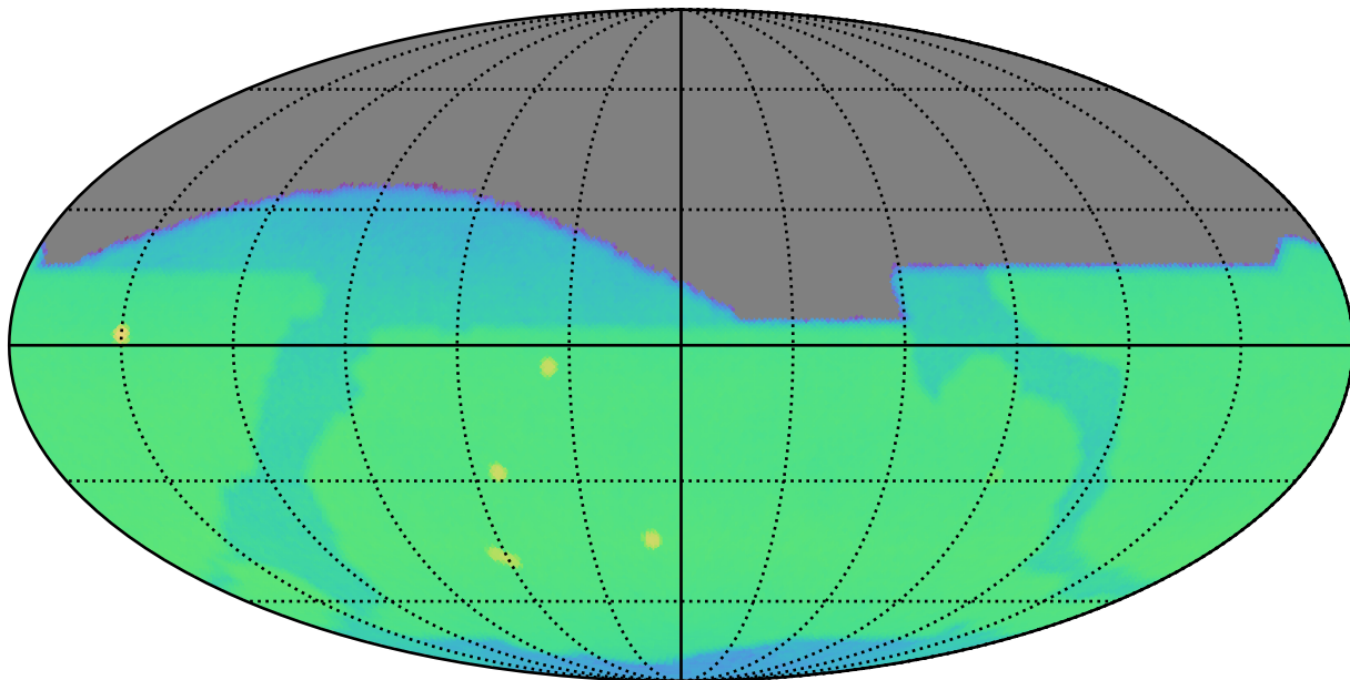
weather_cloudso35v3.5_10yrs r: CoaddM5
