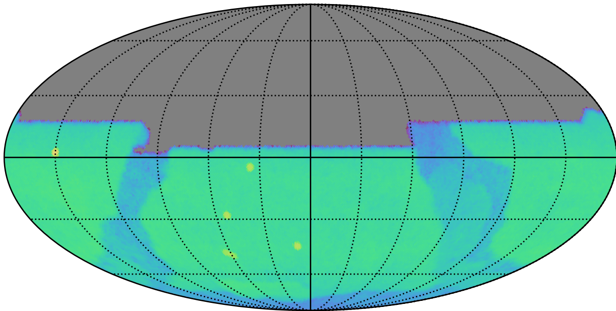
weather_cloudso35v3.5_10yrs u: CoaddM5
