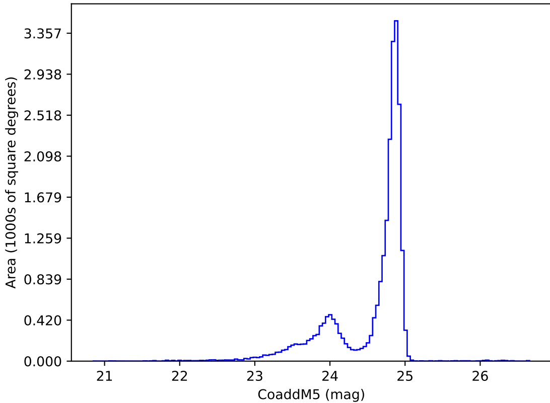
weather_cloudso35v3.5_10yrs y: CoaddM5
