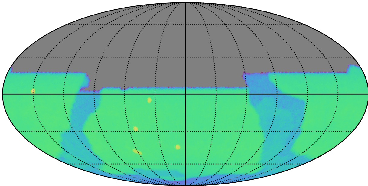
weather_cloudso35v3.5_10yrs y: CoaddM5
