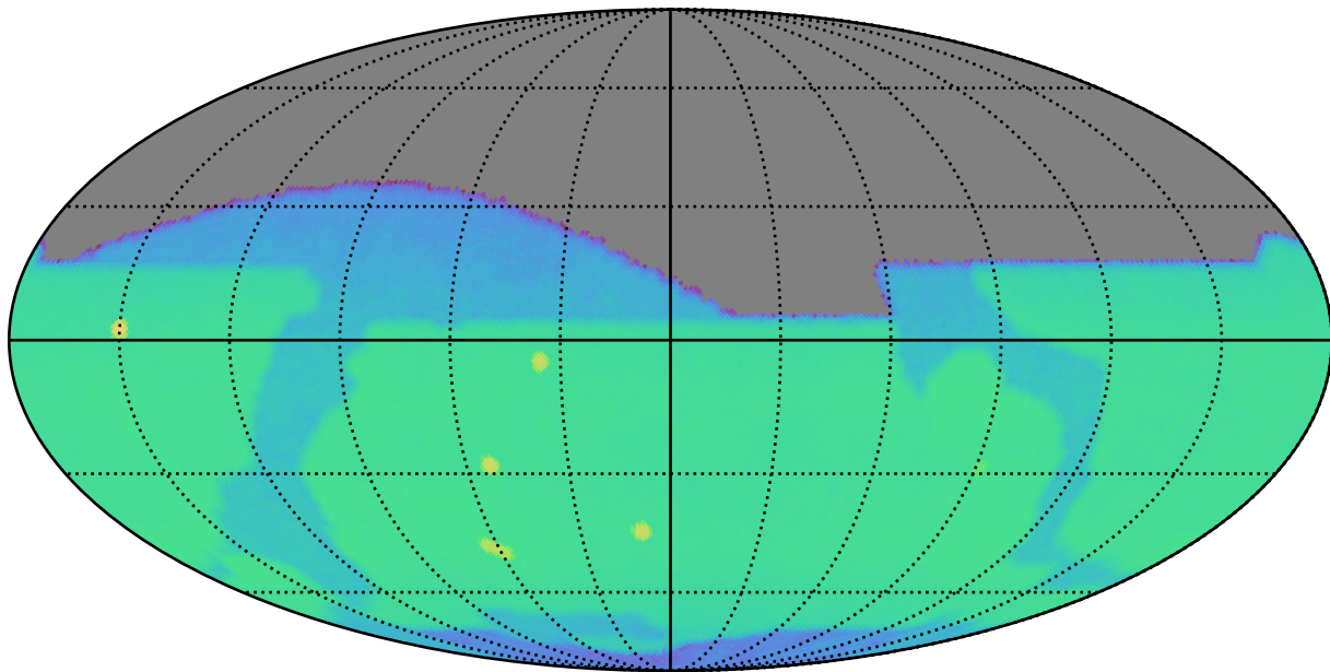
weather_cloudso35v3.5_10yrs z: CoaddM5
