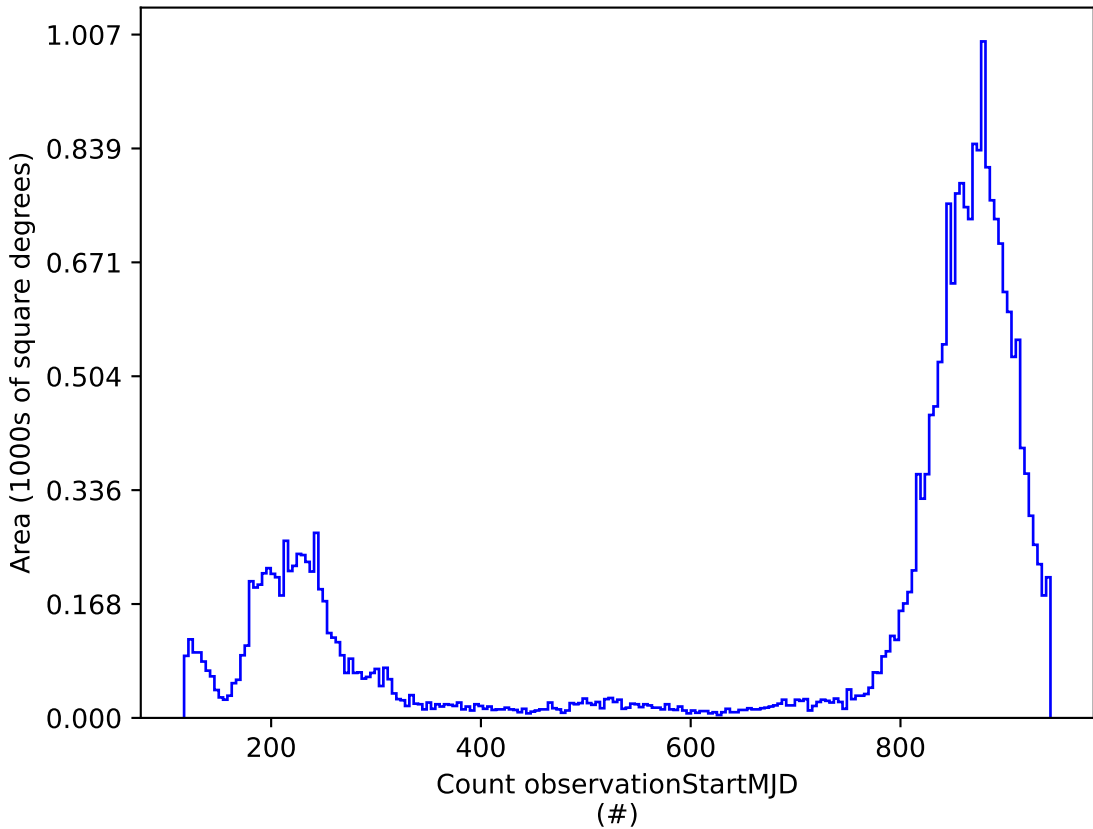
weather_cloudso35v3.5_10yrs : Count observationStartMJD
