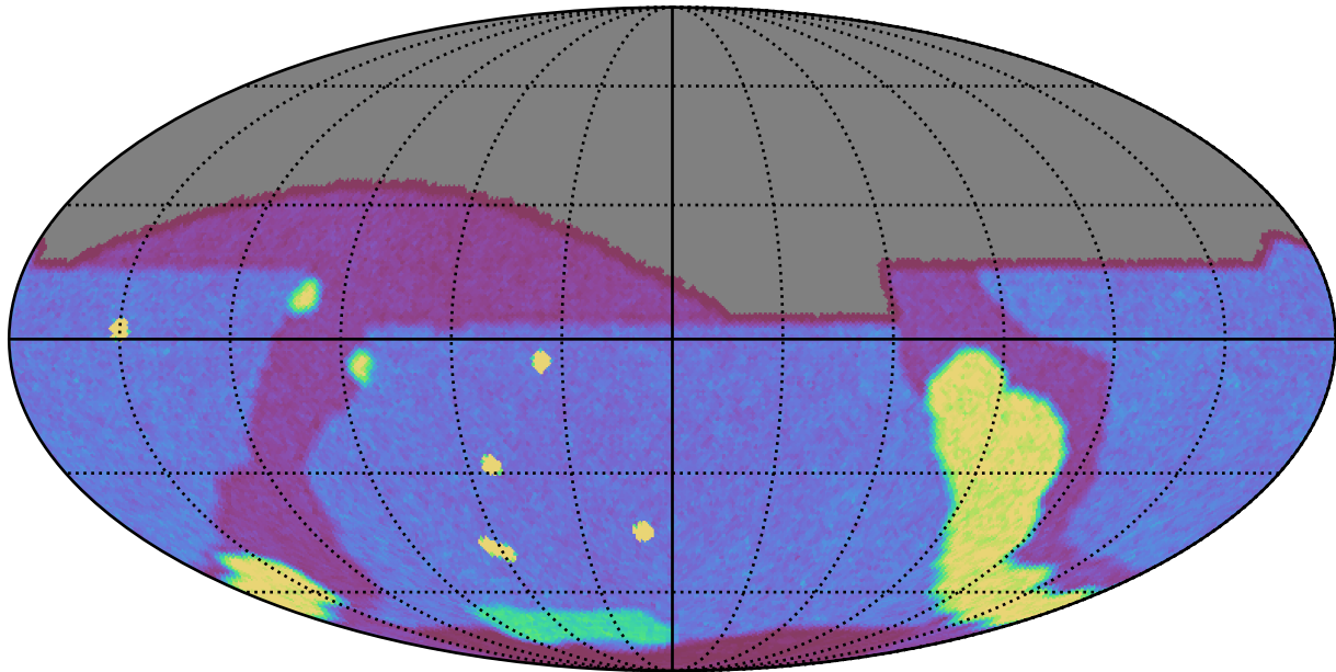
weather_cloudso35v3.5_10yrs g: Count observationStartMJD
