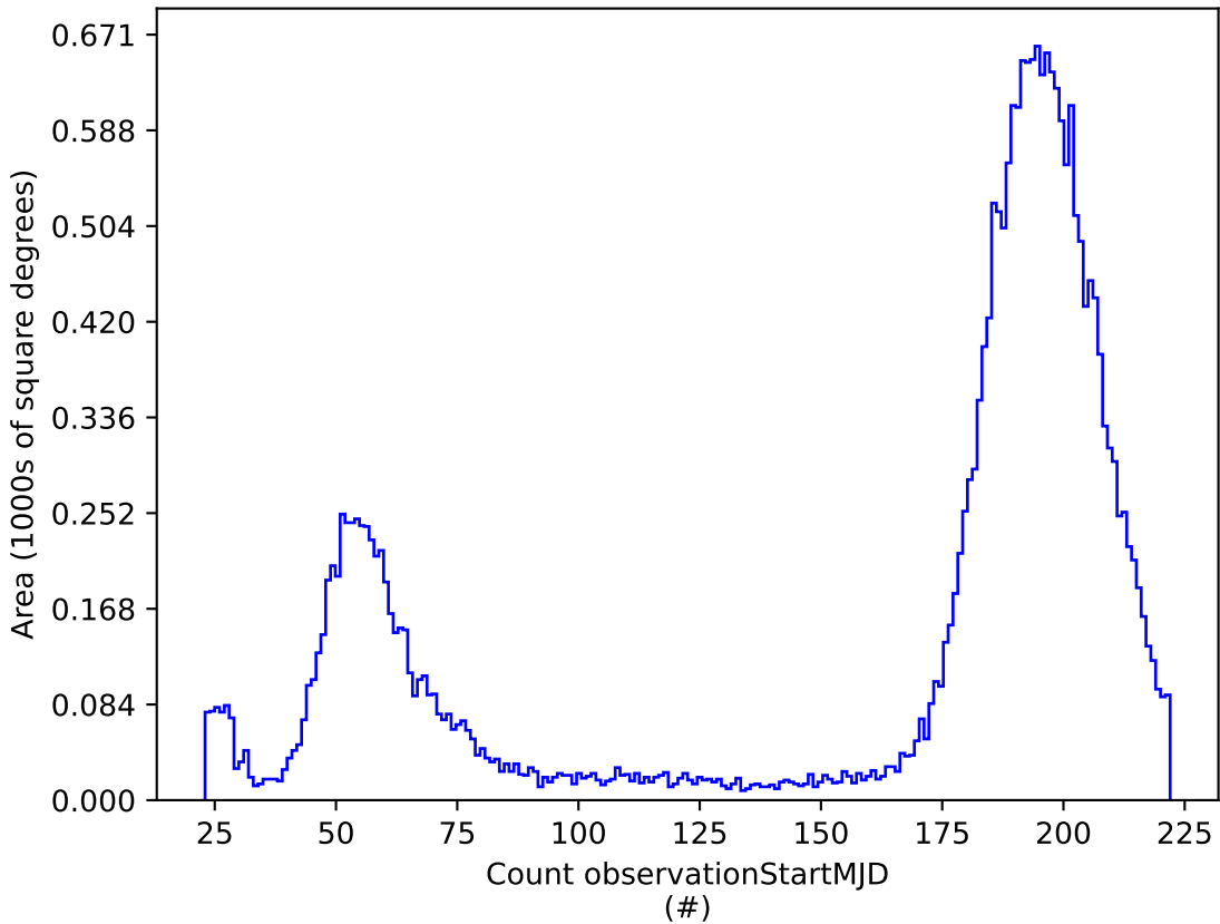
weather_cloudso35v3.5_10yrs i: Count observationStartMJD
