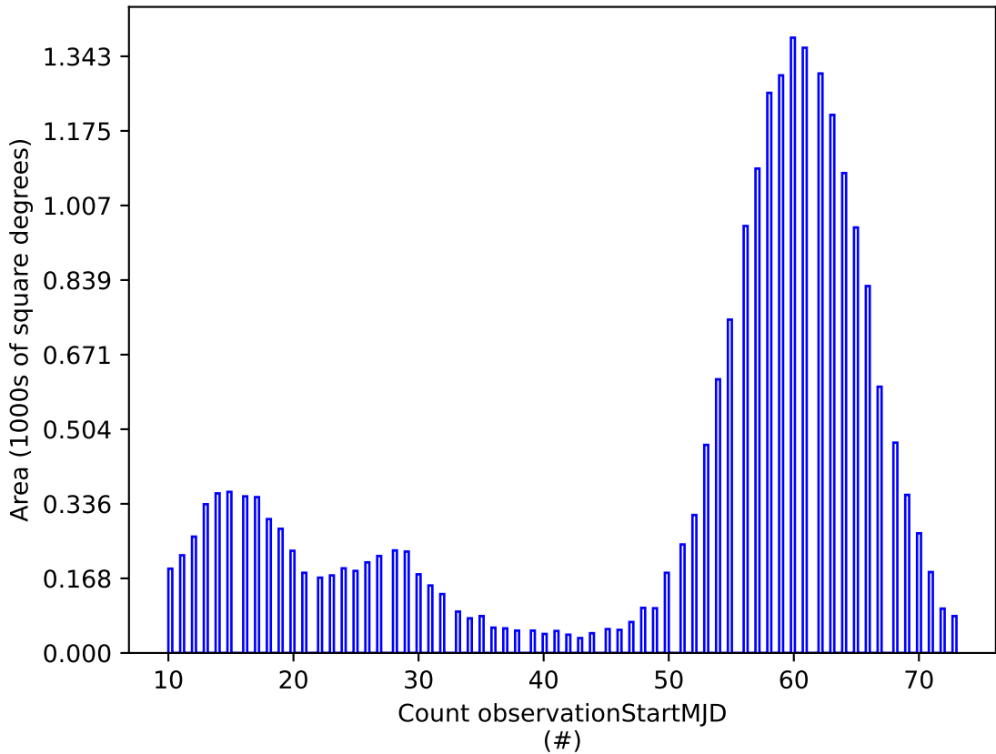
weather_cloudso35v3.5_10yrs u: Count observationStartMJD
