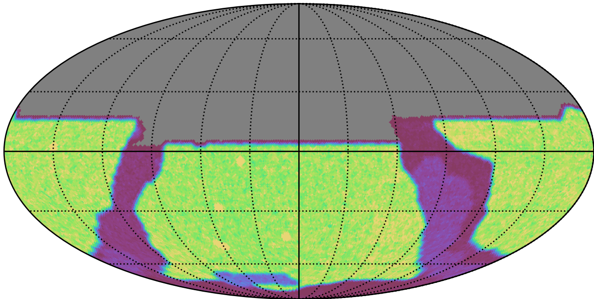
weather_cloudso35v3.5_10yrs y: Count observationStartMJD
