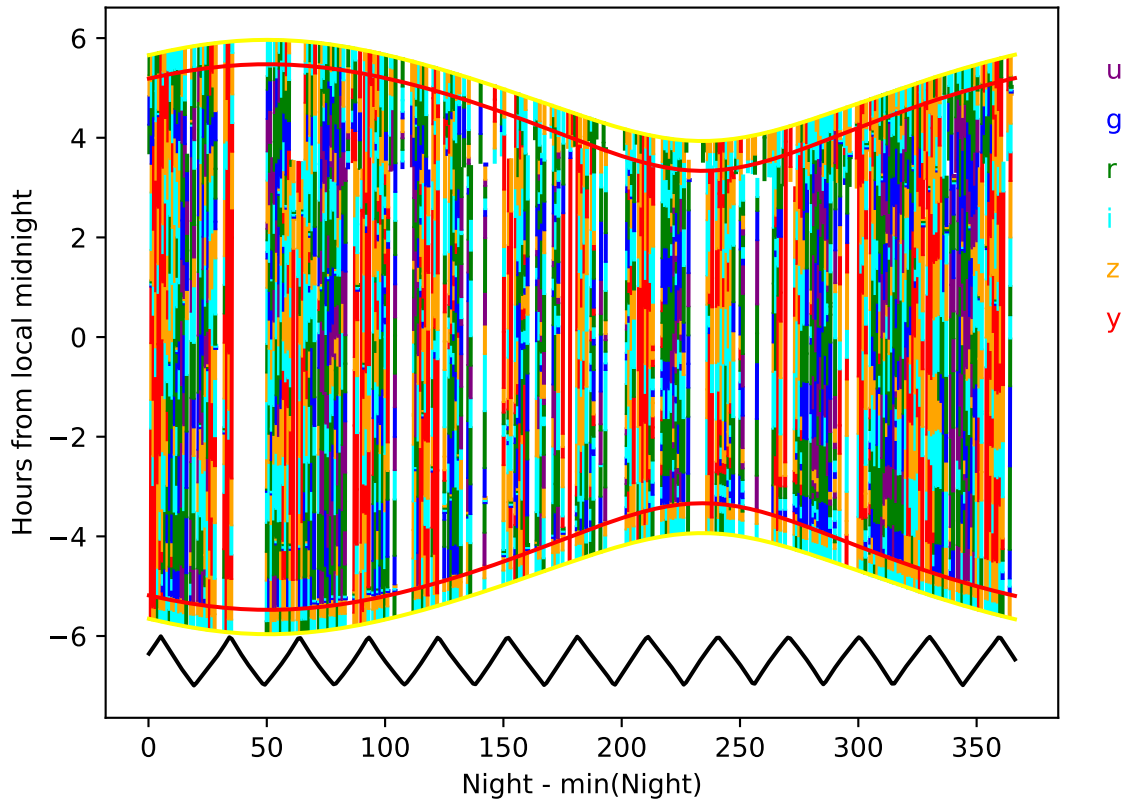
weather_cloudso35v3.5_10yrs year 6-7: Hourglass
