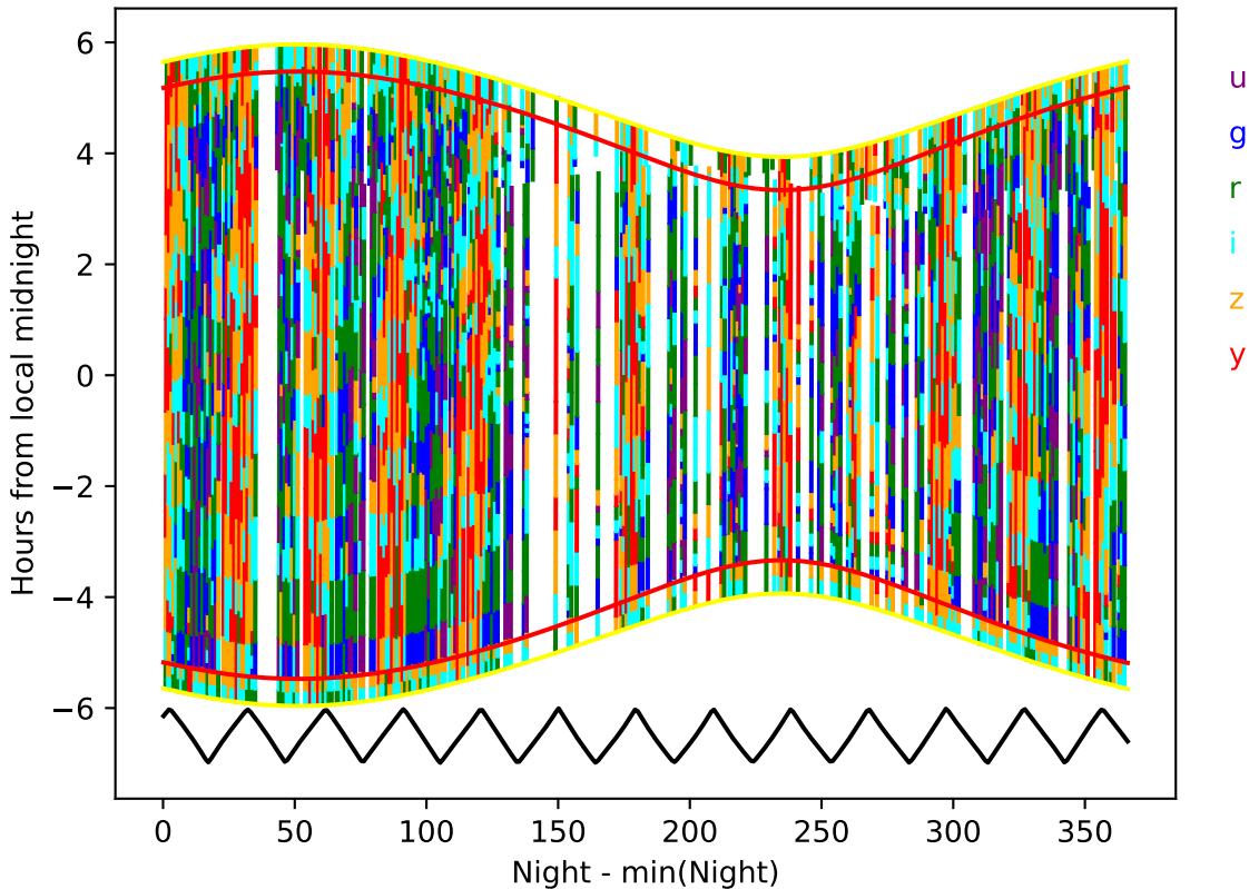
weather_cloudso35v3.5_10yrs year 9-10: Hourglass
