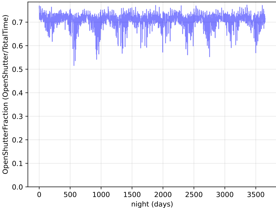
weather_cloudso35v3.5_10yrs : OpenShutterFraction
