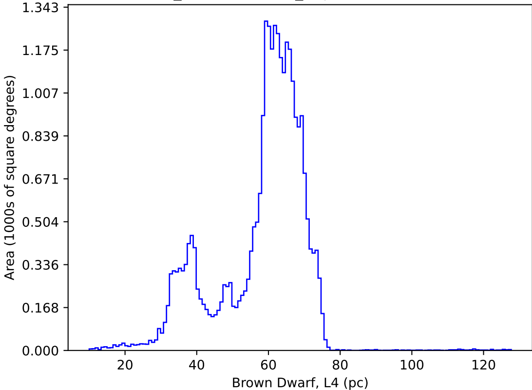
weather_cloudso35v3.5_10yrs : Brown Dwarf, L4
