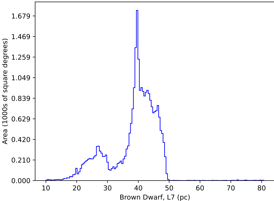
weather_cloudso35v3.5_10yrs : Brown Dwarf, L7
