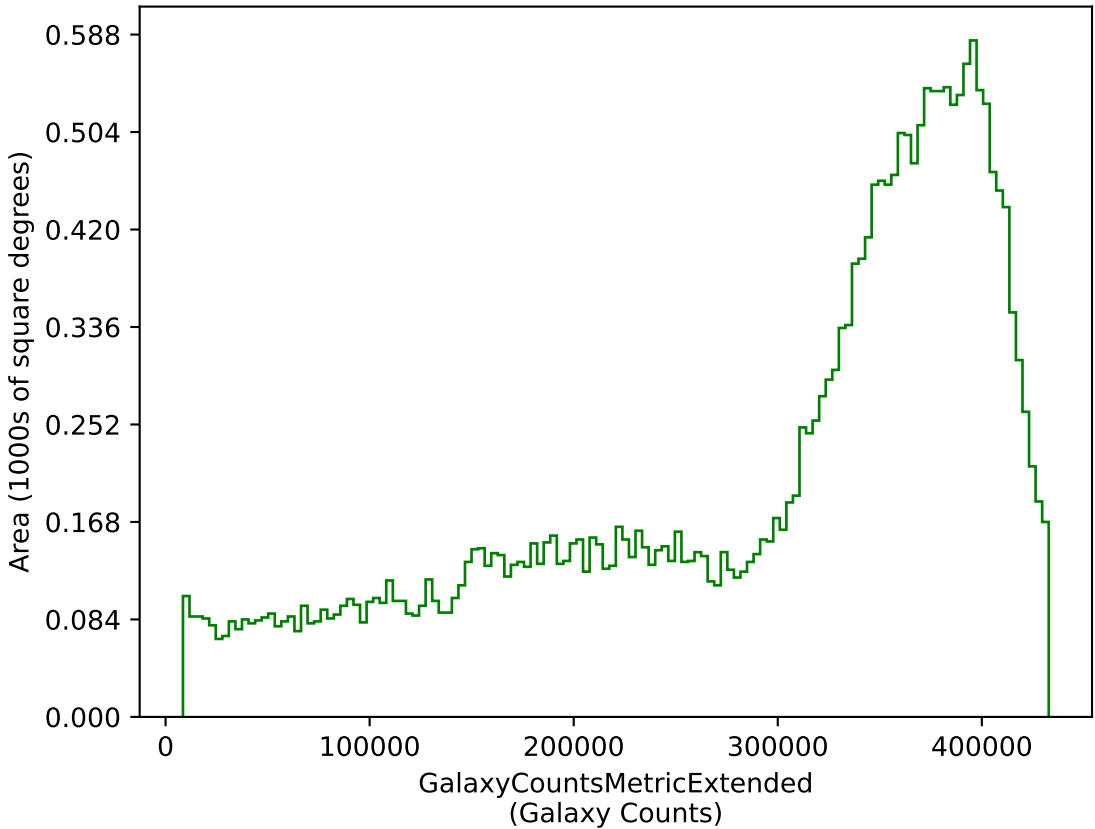
weather_cloudso35v3.5_10yrs g: GalaxyCountsMetricExtended
