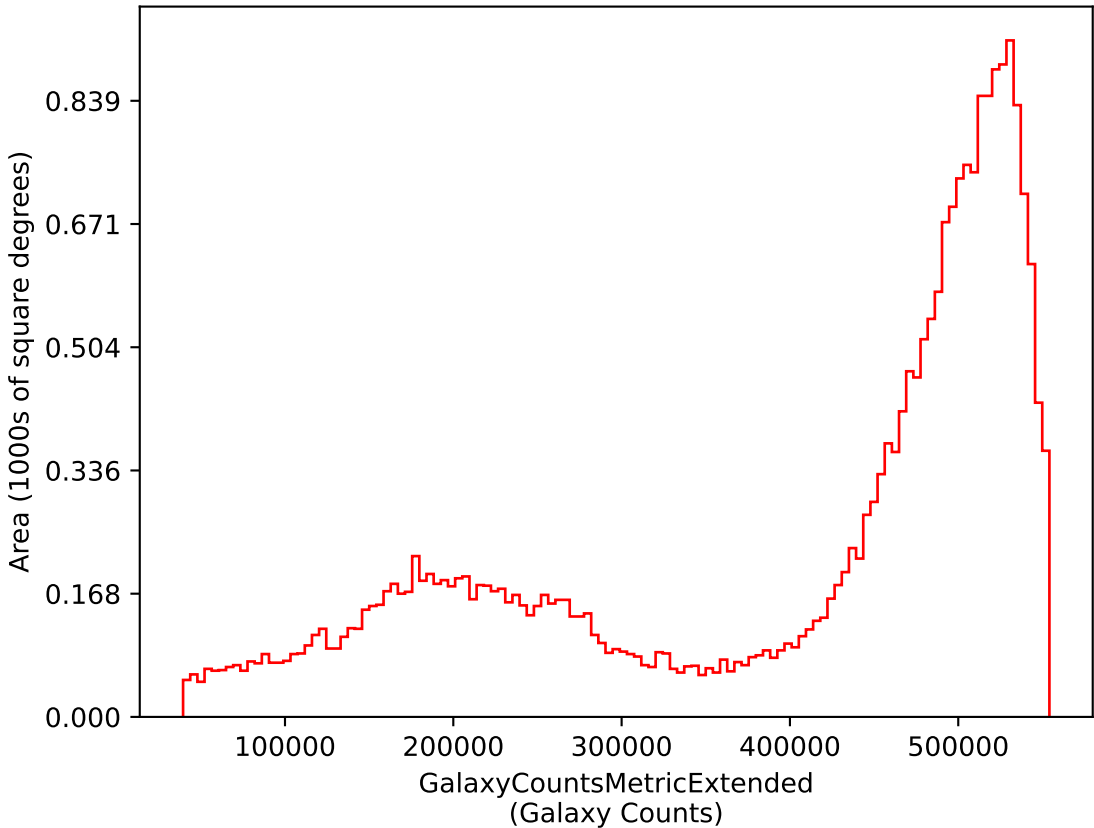
weather_cloudso35v3.5_10yrs i: GalaxyCountsMetricExtended
