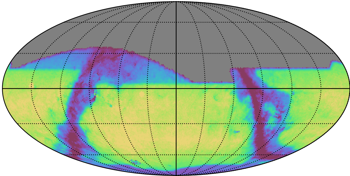
weather_cloudso35v3.5_10yrs i: GalaxyCountsMetricExtended
