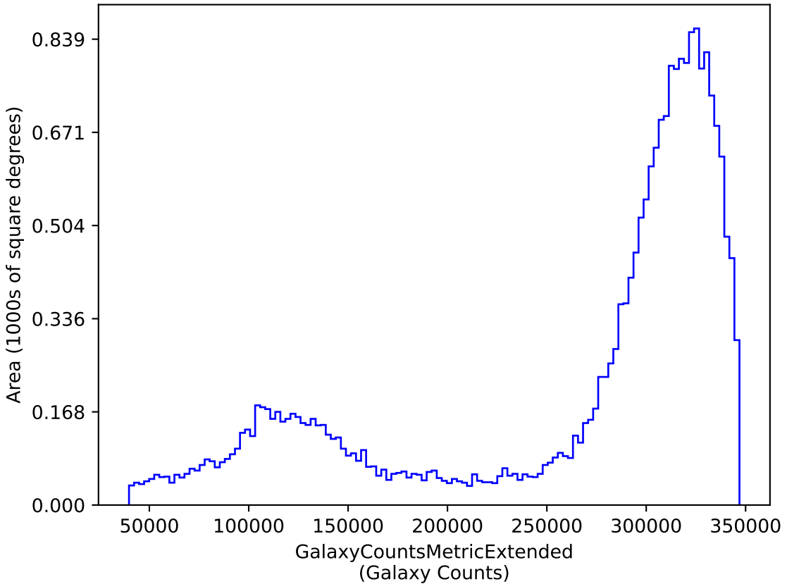
weather_cloudso35v3.5_10yrs y: GalaxyCountsMetricExtended
