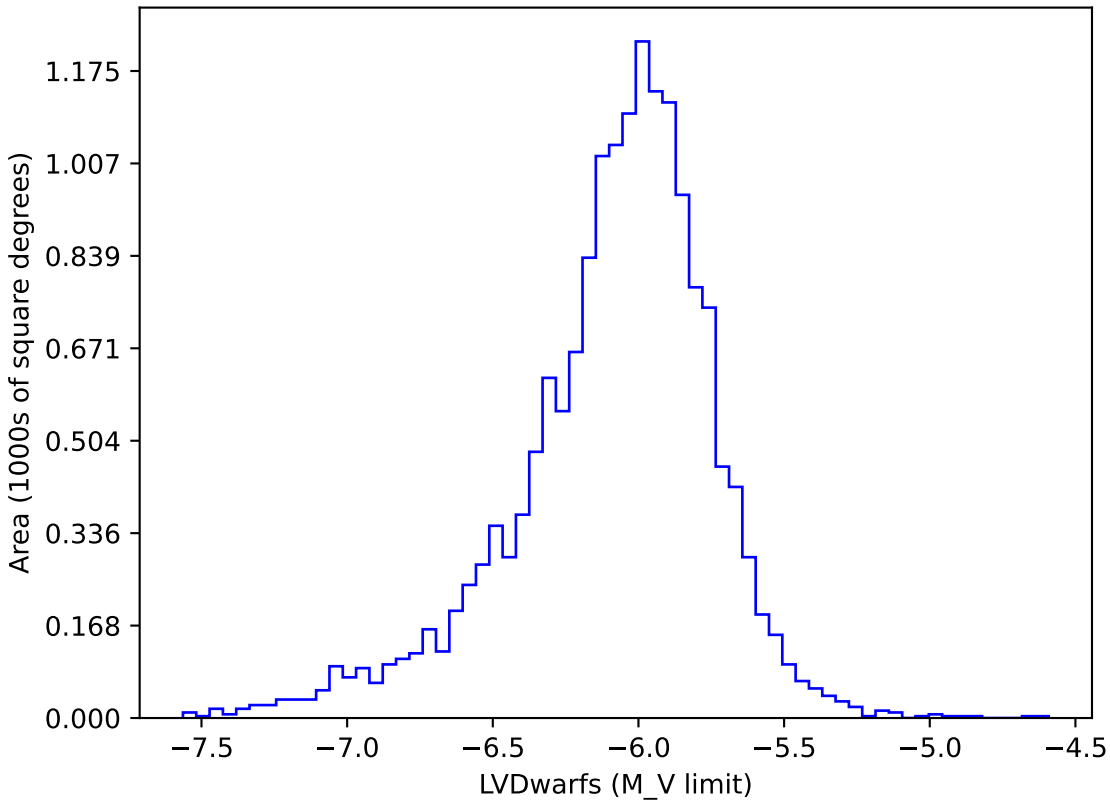
weather_cloudso35v3.5_10yrs gi: LVDwarfs
