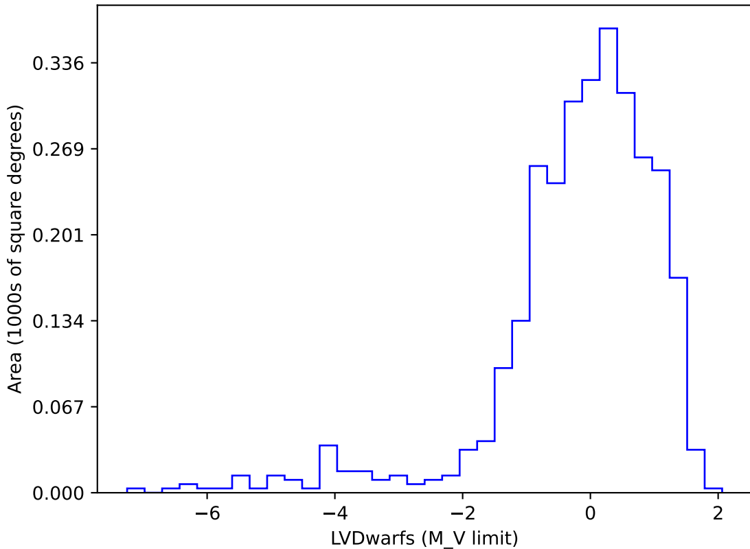
weather_cloudso35v3.5_10yrs gi SCP: LVDwarfs
