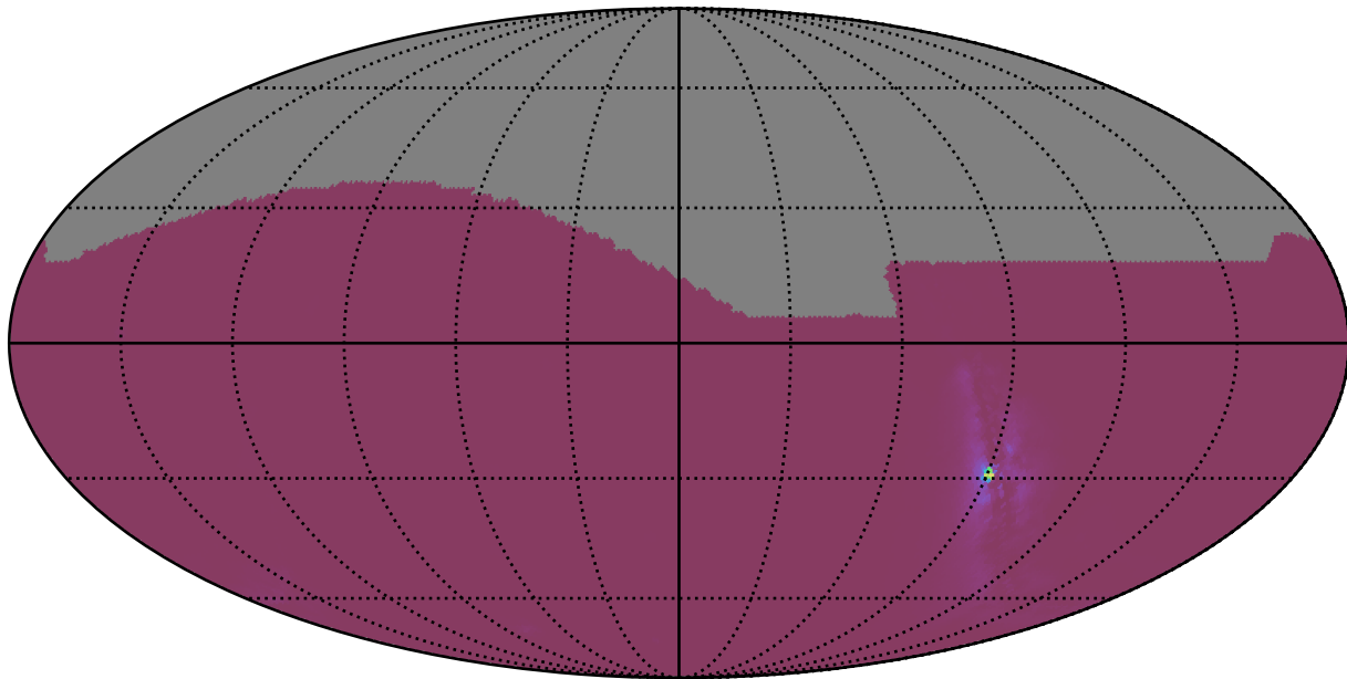
weather_cloudso35v3.5_10yrs : NlcPoints
