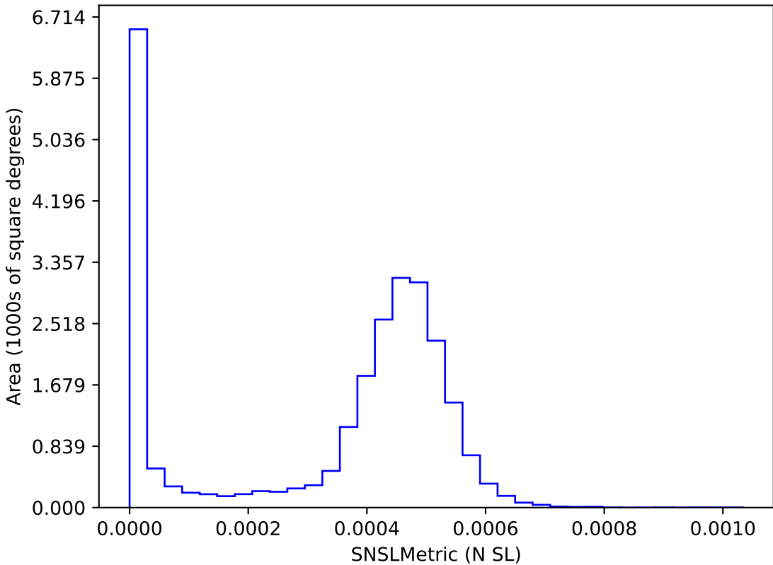
weather_cloudso35v3.5_10yrs : SNSLMetric
