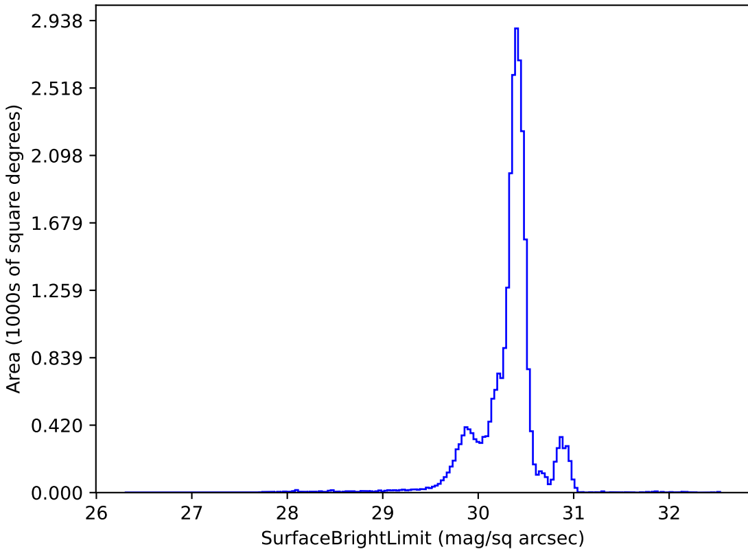
weather_cloudso35v3.5_10yrs g: SurfaceBrightLimit
