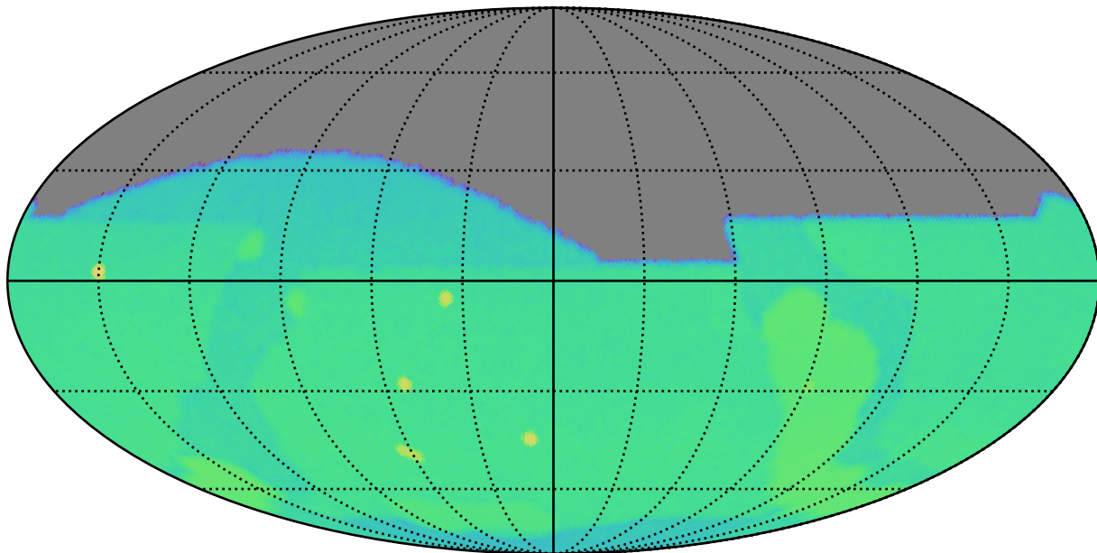
weather_cloudso35v3.5_10yrs g: SurfaceBrightLimit
