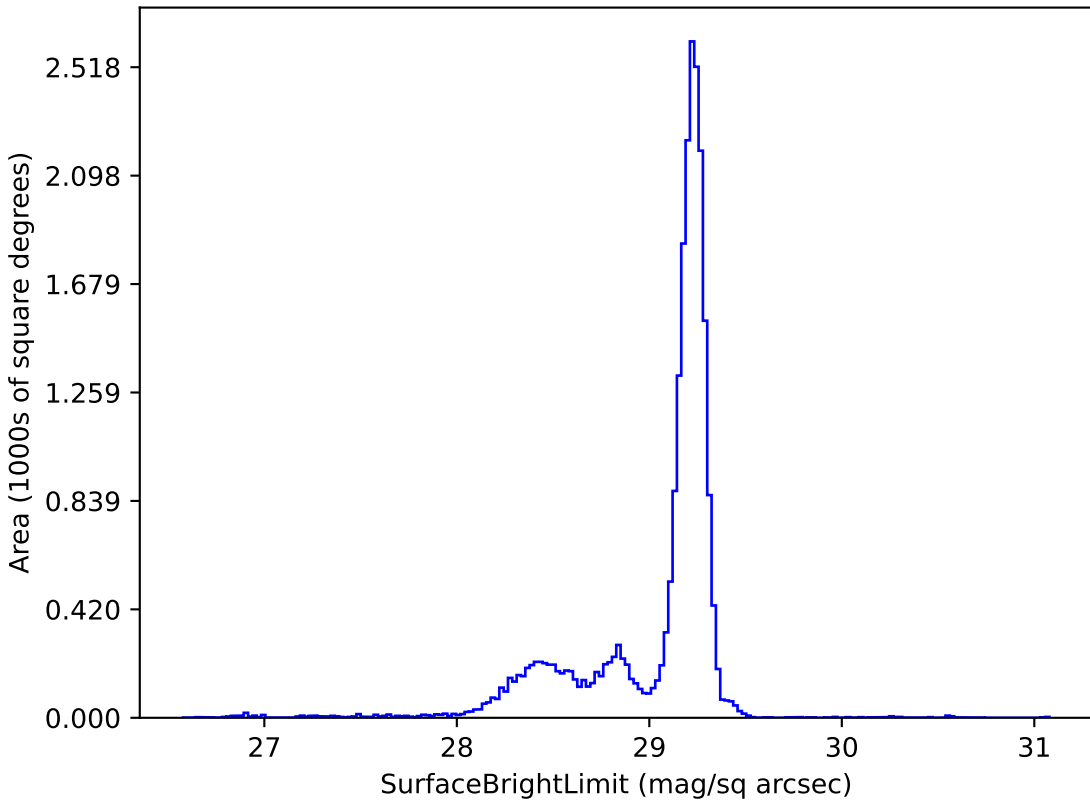
weather_cloudso35v3.5_10yrs u: SurfaceBrightLimit
